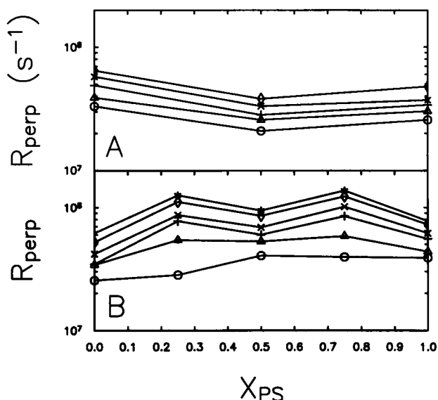
FIGURE 6 Semi-log plot of R_{\perp} of CSL as a function of mole fraction of POPS, x_{PS} , in POPC/POPS mixtures at various temperatures. (A) CSL. \circ , 35°; \Delta , 43°; + , 51°; \times , 59°; \diamond , 67°. (B) 5-PC. \circ , 25°; \Delta , 35°; + , 45°; \times , 51°; \diamond , 61°; * , 68°.
